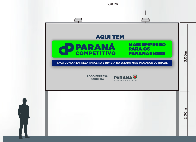
Vista frontal
